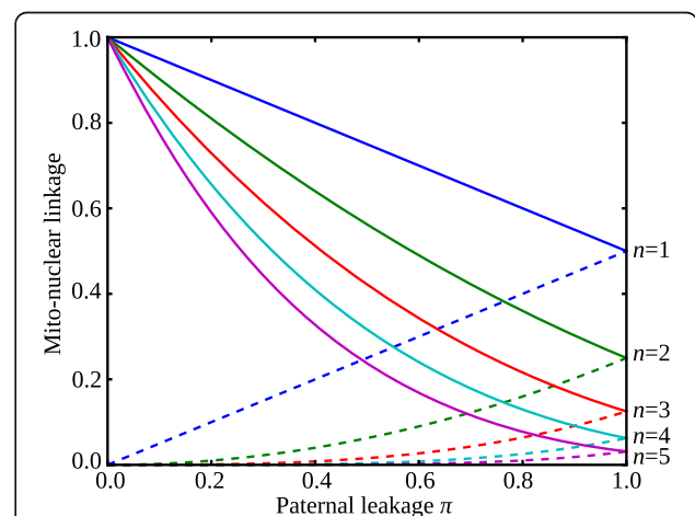
Fig. 4 Strength of mito-nuclear statistical association (linkage). Linkage measured as the proportion of mitochondria after n generations that are identical by descent to those at generation n = 0 . Solid curves represent linkage under maternal nuclear control of mitochondrial inheritance, while dashed curves correspond to paternal control. The two modes of control differ in the way that paternal leakage affects the strength of mito-nuclear associations over time. For maternal control, the linkage is (1 - \frac{\pi}{2})^n and declines with \pi , as with increasing paternal leakage fewer maternal mitochondria are passed on to each offspring. For paternal control, the linkage strength is (\frac{\pi}{2})^n and increases with \pi , as with higher values of paternal leakage more paternal mitochondria are transmitted to the zygote
